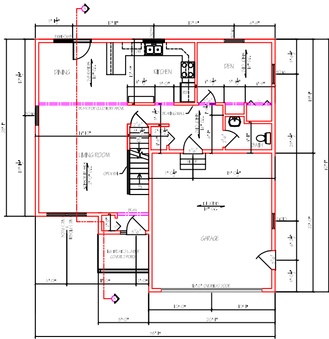
FIRST FLOOR PLAN SCALE: 1/4" = 1'
