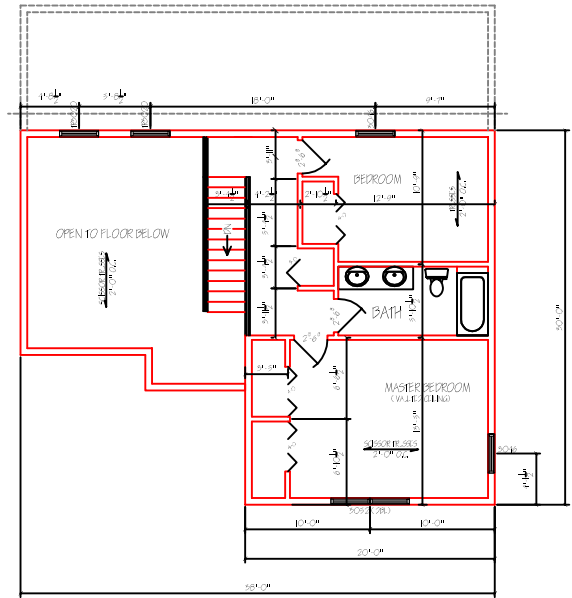
SECOND FLOOR PLAN SCALE: 1/4" = 1'
