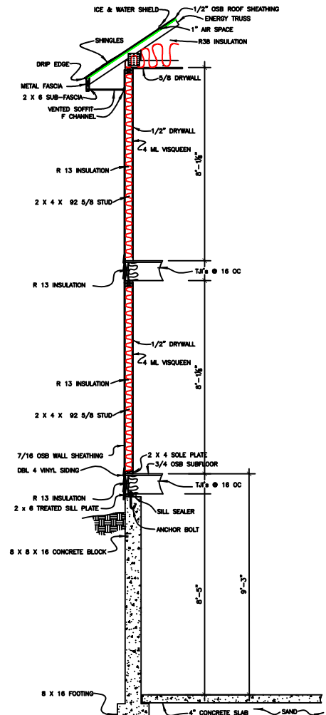
TYPICAL SLAB WALL DETAIL
