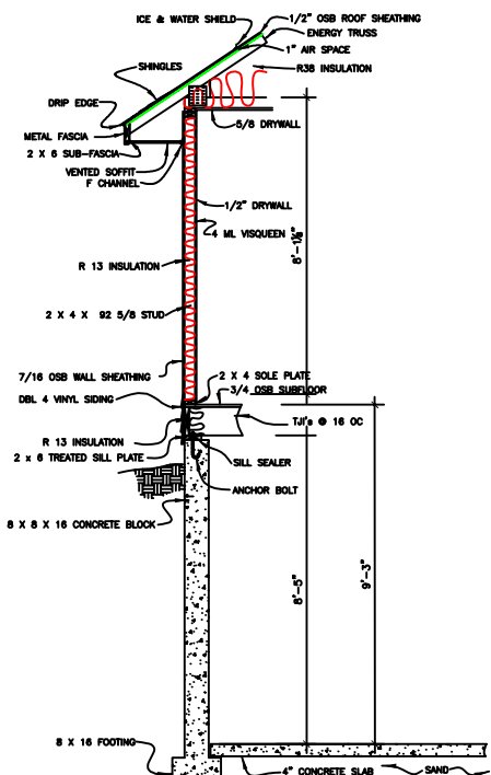
TYPICAL WALL DETAIL
