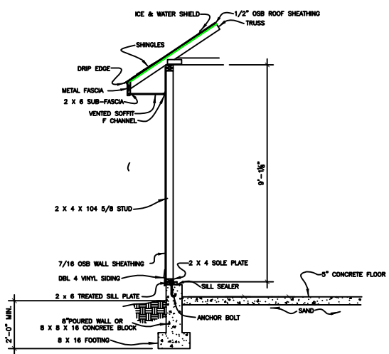
TYPICAL GARAGE WALL DETAIL
